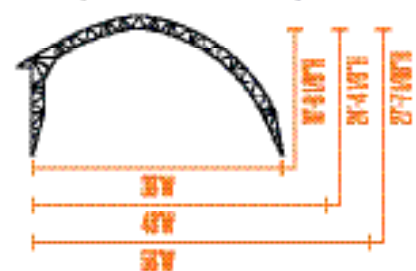
ClearSpan Commodity Buildings
